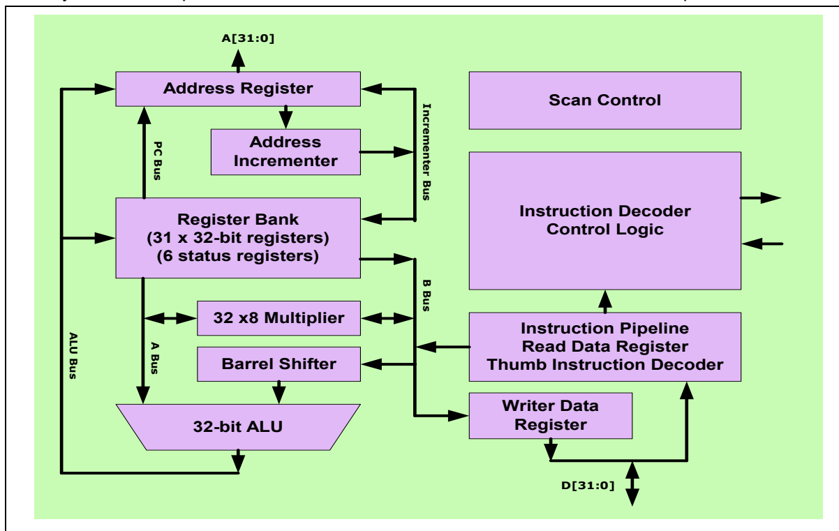
Fig 6.1 ARM7TDMI CPU Core Block Diagram
