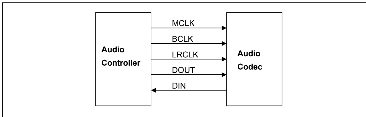
Figure 6.11.2.1 The interface signal of IIS
